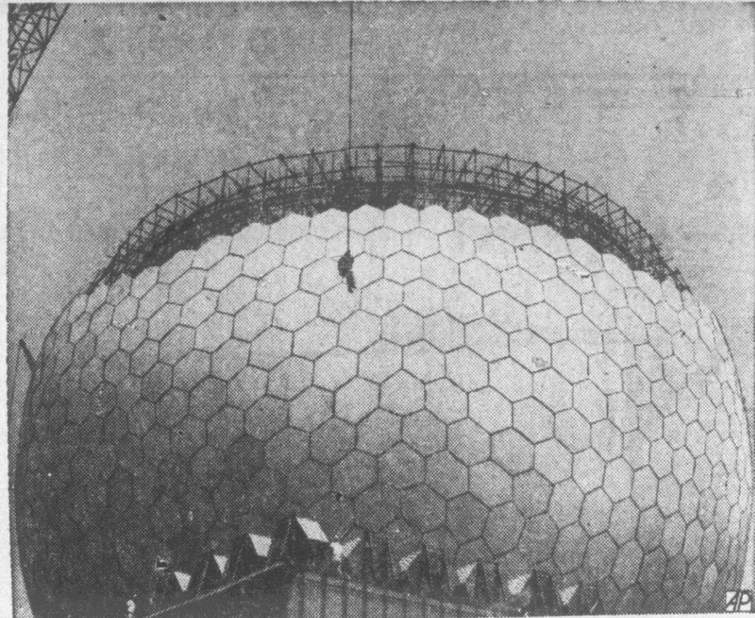
SECTIONAL SIGHT—Work progresses on dome, 140 feet in diameter, being built at Moorestown, N. J. Structure, made of paper pressed into hexagonal plates, is a prototype for domes to be built for Air Force use in an Arctic early warning system.
