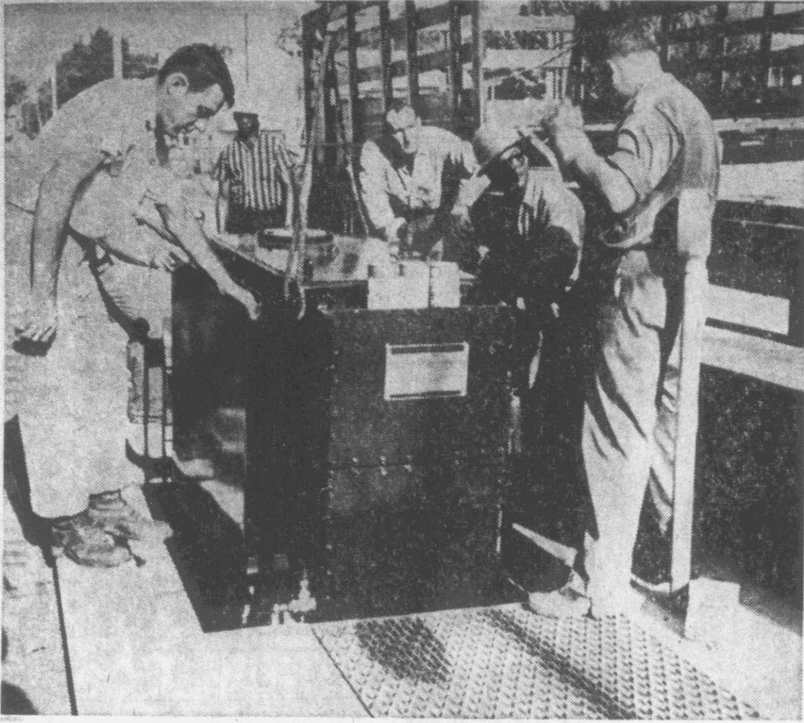
NEW TRANSFORMER —Workmen are shown lowering a 7,400 pound 12,000 volt network transformer into the recently constructed underground transformer vault on Fifth St. near the Municipal building. The 500 KW unit will supply current to the area and to a new building being constructed across the street. A 2,200 pound network protector is also being installed on the transformer. No cost estimate could be obtained on the installation this morning.
