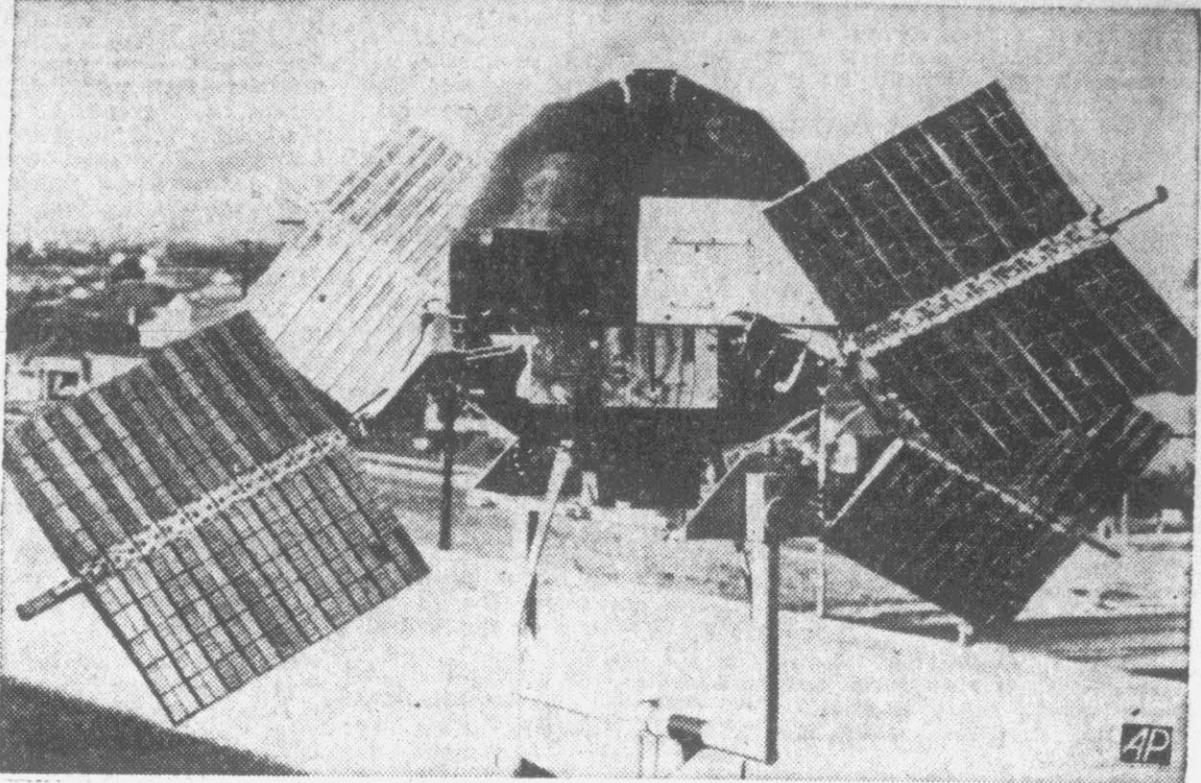
"PADDLEWHEEL" SATELLITE SOARS IN ORBIT—Here's the 142-pound "paddlewheel" satellite which was launched at Cape Canaveral, Fla., Friday and soared into orbit. The Space Agency said it will remain aloft more than a year. The four solar vanes, which give the satellite its name, are designed to pop out from sides in space to convert the sun's rays into electrical energy for the enclosed radio transmitter batteries. This creates the satellite's own power for transmitting information back to earth. The "paddlewheel" is packed with instruments and serves as a flying laboratory exploring the mysteries of space. (AP Wirephoto)
