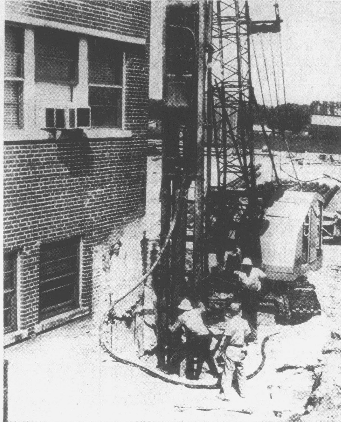
PILE DRIVER . . . at Pitt Memorial Hospital this morning started driving the 74 piles needed for the one-story west wing addition to the building. The 40-foot long piles are driven down by a 5,000 pound steel hammer that strikes the metal pilings with a force of 15,000 pounds per square inch when forced down from a height of three feet by air pressure. A total of 216 piles will be driven, including 16 for the new administrative wing and 126 for the four-story wing at the rear of the building. Completion of the one-story west wing is expected in from six to eight months.
