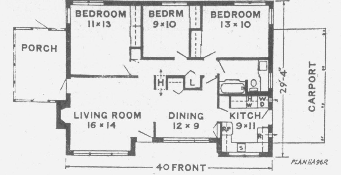
ON A SLAB: This seven room Florida-type home is designed for construction on a slab. It has three bedrooms. The plan is HA96R by Architect Jan Reiner, P. O. Box 96, New Port Richey, Fla. The habitable area is 1,130 square feet.
