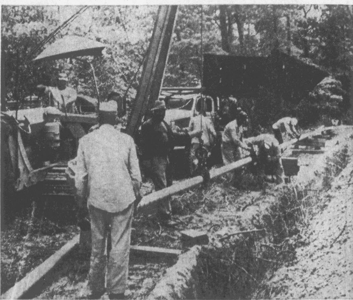
NATURAL GAS PIPELINE—Under ideal conditions, workers can lay two miles of this four-inch line per day. The 35-foot to 55-foot long sections are welded together, their joints tarred and then placed in the ground. Workers near the intersection of 14th St. and U. S. 264 laid 7,400 feet of line yesterday. They are expected to place a line four and one-half feet under the bottom of Tar River within the next two weeks. All lines are tested under 1,000 pounds pressure for a period of from 24 to 48 hours before they are put into service. (Reflector Staff Photo)
