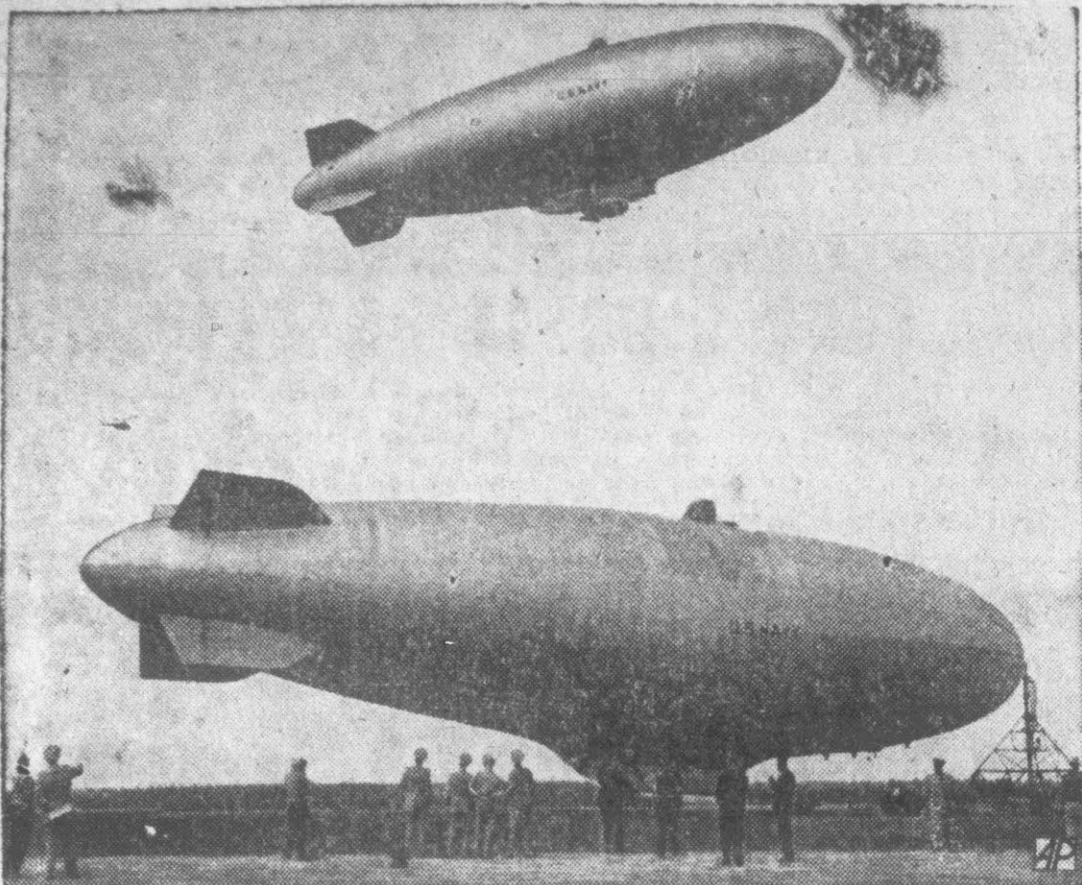
CASEOUS MOORING —Navy's largest new dirigible is anchored at Lakehurst, N. J., as smaller ship passes by. Over million cubic feet of helium fill 493-foot bag.
