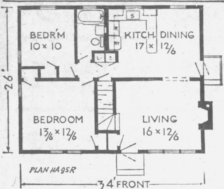
ECONOMY HOUSE: This tiny home has two bedrooms down stairs, and room for two more and a bath in an expansion attic upstairs. The square foot area of the first floor is 884 sq. ft. The plan is HA95R by Architect Jan Reiner, P. O. Box 96, New Port Richey, Fla.
