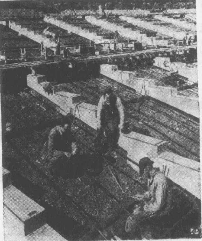
SEAT-SETUP — Workmen weld iron pipes for radiant heating system which will warm the reserved seat section of Giants' new Candlestick Park in San Francisco.
