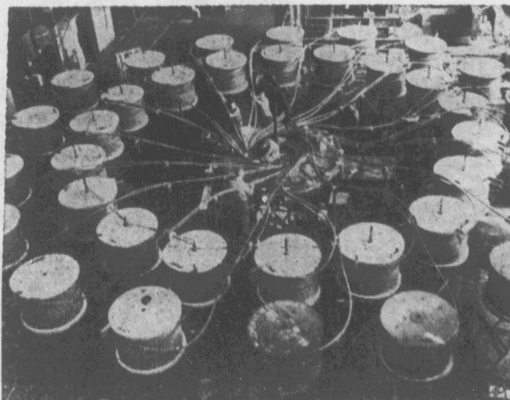
BIG SCALE WINDUP — Reels feed copper cable to workmen winding huge induction coils at Pittsfield, Mass., plant. Finished coil weighing 60 tons will be used as part of an electrical power supply system for an Air Force hypersonic wind tunnel.
