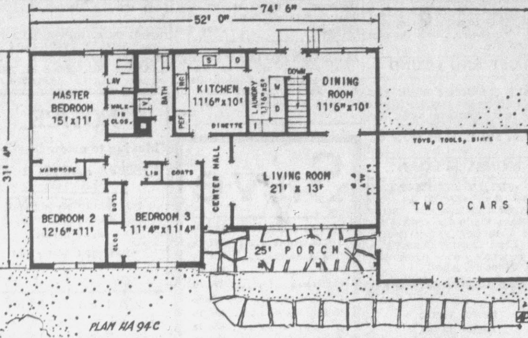
COLONNADE PORCH: An inviting porch is the main architectural feature of this charming three-bedroom ranch. The plan is HA94C, by Architect Lester Cohen, Rm. 75, 117 West 48th St., New York 36, N. Y., and has a floor area of 1,484 sq. ft., excluding garage.
