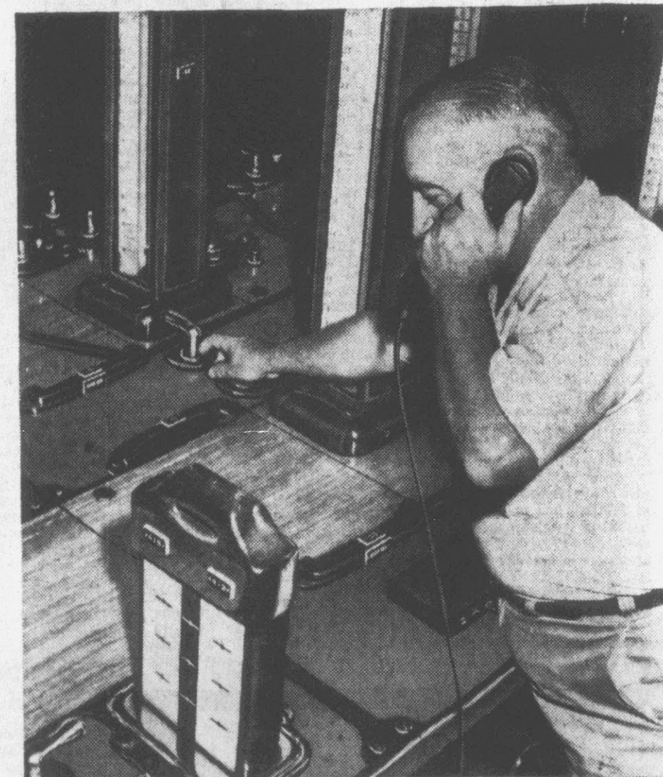
Lockmaster Richard Abel, on lock wall, phones an order to the Miraflores Locks control tower. . . and, in tower, Frank Dolan, control house operator, throws small switch to swing open the 750-ton gate leaves.
