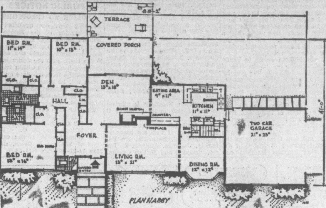
TWO LIVING ROOMS: An oversized den, with a fireplace of its own, gives this luxury home two living rooms. The architect also has provided three bedrooms, full dining room and efficient U-shaped kitchen. The habitable area is 2,007 square feet and the plan is HA88Y by Architect Herman H. York, 90-04 161st St., Jamaica 35, New York.
