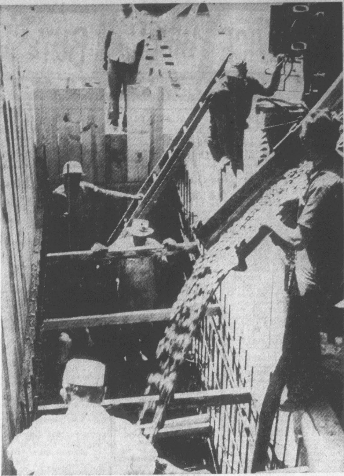
VAULT FLOOR BEING POURED—Workmen are shown pouring the floor for a sidewalk transformer vault now under construction on West Fifth St. beside the Municipal Building. (Reflector Staff Photo)
