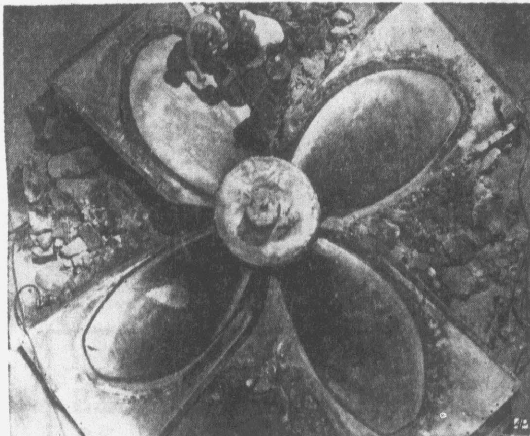
KING-SIZE PROP — What appears to be a giant four-leaf clover is in reality a 55,000-pound ship propeller being removed from mould after casting at San Francisco.
