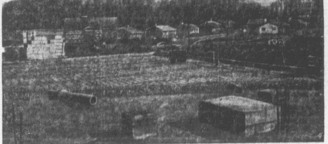
PIER SLAB—Here's a cross-sectional view of the intermediate pier slab system under construction. Each of the two 16" square piers showing is matched by two more in line under the vapor barrier and welded wire fabric. The large, rectangular concrete block structure between the piers is the base for a furnace. Heat ducts run under the slab.
