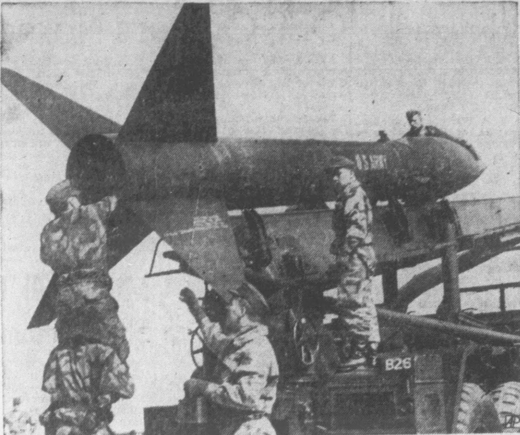
STRAIGHT AIM — West German soldiers ready an Honest John tactical rocket at Eschweiler army base. The first operational rocket group will be ready shortly.
