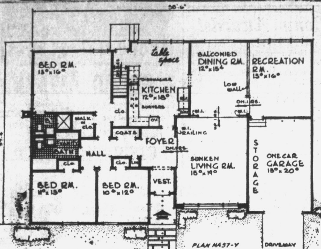
A SUNKEN LIVING ROOM and a dropped recreation room are interior features of this one-story ranch. And, welcome news to mother, the kitchen is 18 feet long with an outside door for a service entrance. The plan, HA57-Y, is by Architect Herman H. York, 90-04 161st St., Jamaica 32, New York. Excluding the recreation room, the main level has 1,644 sq. ft. The recreation room has 216 sq. ft. and the garage 275 sq. ft.
