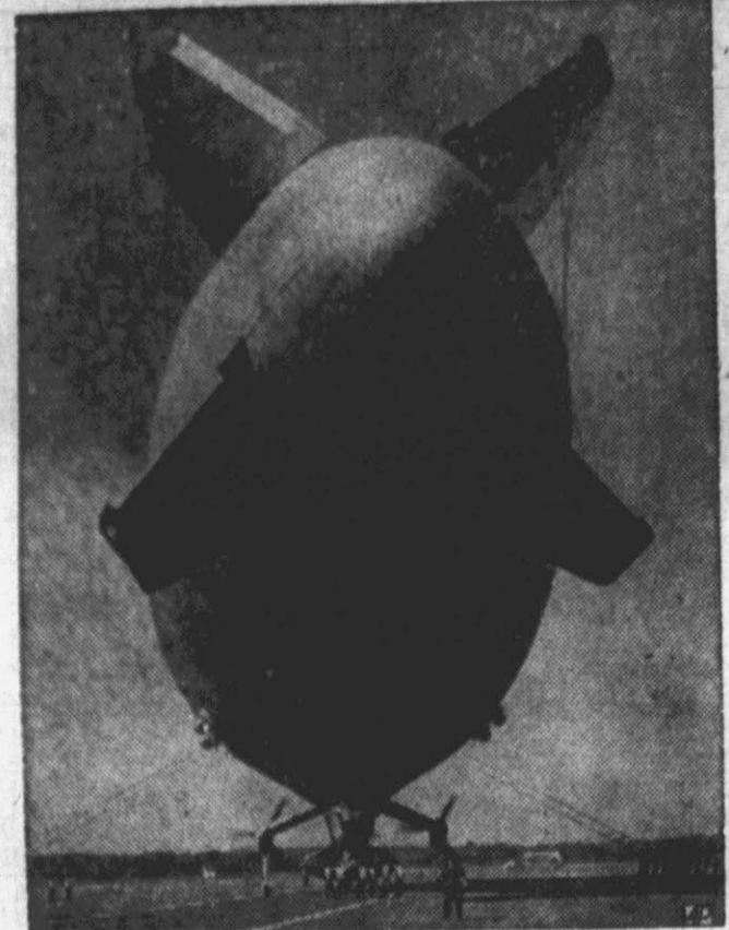
BACK TO BASE—The U. S. Navy blimp ZPG-3 lands at Weymouth, Mass., air station after trip to Arctic to test use of similar craft for research in polar areas.
