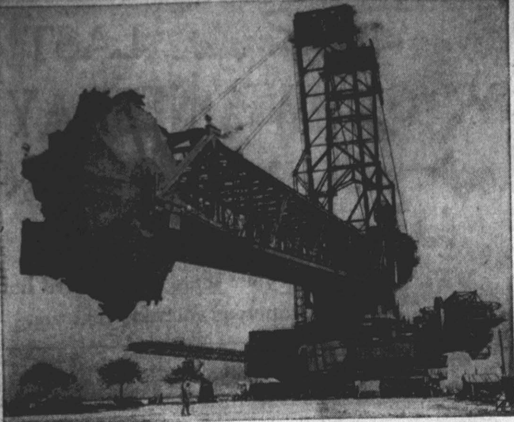
GIANT ON THE MOVE — This 6,000-ton dredging machine looms above the landscape at Duerwis, Germany, as it lumbers under its own power to a nearby job. The huge digger, built in two years, has an overall length of more than 500 feet and is over 200 feet high.
