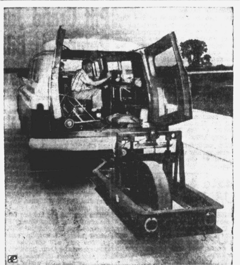
TEST ON LEVEL —An engineer works instruments on truck as an electronic "smoothometer" charts profile of pavement on Illinois highway. The device is used in removal of bumps.
