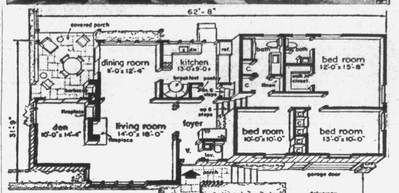
A SIDE TO SIDE SPLIT LEVEL, this house has nine rooms, including three bedrooms, and two baths. There are 1,614 sq. ft. in the habitable area. The area under the bedroom wing, not shown in the floor plan, includes laundry room, garage and recreation room. The plan, HA37-T, is by Designer Edward R. Tyler, 586 Macon Place, Uniondale, N. Y.
