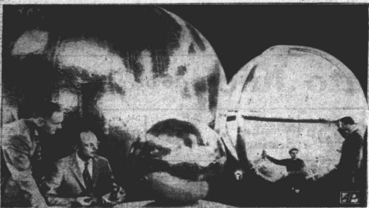
BALLOONS DESIGNED FOR SPACE—These aluminum balloons will be placed in orbit soon to measure density of outer air, the Reynolds Metal Co. announced in Washington. The balloon at left is 12 feet in diameter, and there are a 30-inch and a 12-foot "corner reflectors." Spheres' designer William J. O'Sullivan (second from left) of the National Advisory Committee for Aeronautics holds a collapsed 30-inch sphere. It was made from 65 cents worth of aluminum foil and will go up with one of the next Vanguard satellites. (AP Wirephoto)
