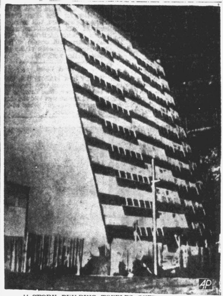
11-STORY BUILDING TOPPLES OVER—Like a child's tiny playhouse, this newly constructed 11-story building topples from its foundation at Rio de Janeiro, Brazil. The unoccupied structure fell on its side a few moments after this picture was made. No one was injured. The collapse was blamed on weak cement in the foundation. (AP Wirephoto)
