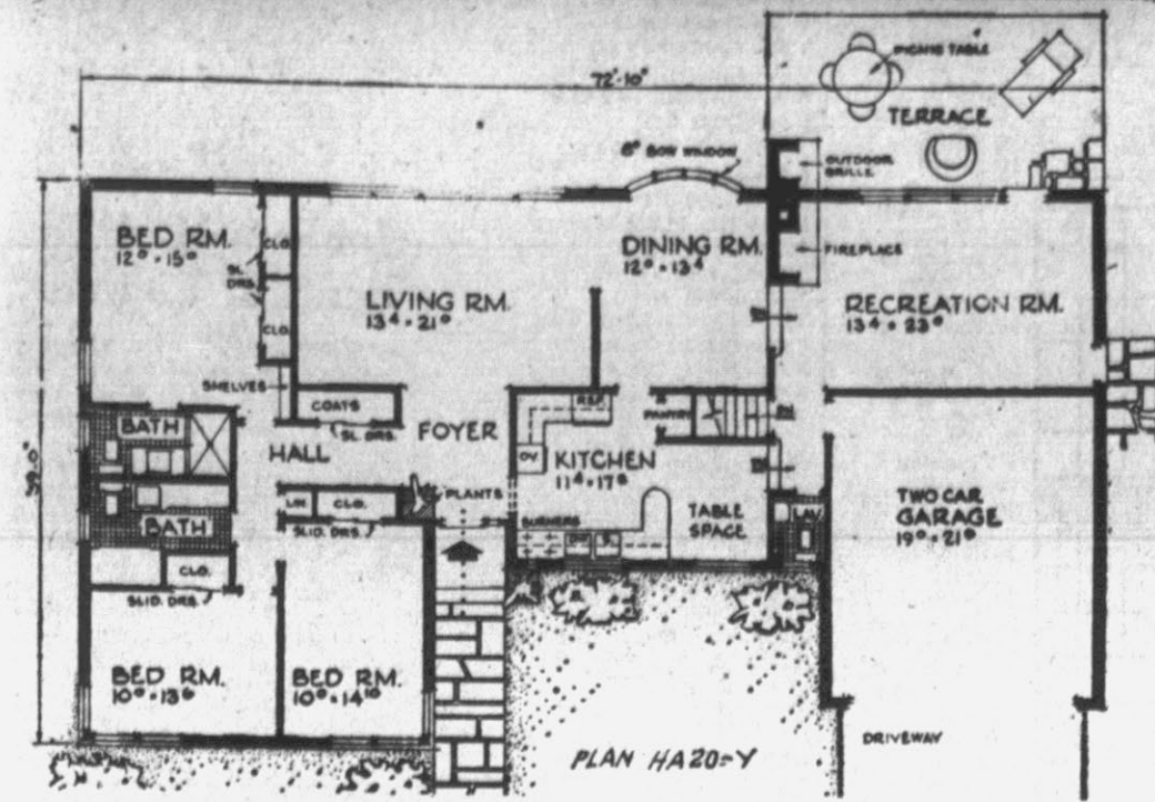
THIS ONE-STORY MODIFIED RANCH HOUSE has seven rooms, two bathrooms and a lavatory room, including three bedrooms, a full basement and a two-car garage. The habitable area has 1,668 sq ft excluding the recreation room and the garage. These areas add 744 sq ft. All of its principal rooms are toward the privacy of the rear outdoor-living area. The plan, HA20-Y, is by Architect Herman H. York, 90-04 161st St., Jamaica 52, N.Y.
