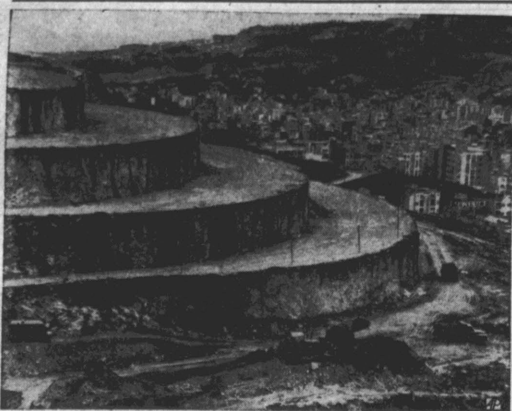
MAN MADE PYRAMID — Spiral roadway, cut into mountainside in Caracas, Venezuela, will give shoppers direct access to heliport-shaped building to be constructed on the site.
