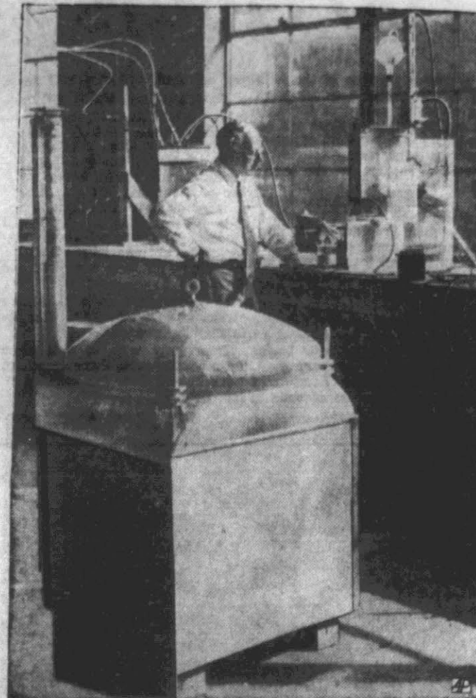
LEGAL STILL: Dr. Kenneth C. D. Hickman patiently waits for his vapor compression still (foreground) to turn salty brine into fresh water. The machine has a capacity of 500 gallons a day.
