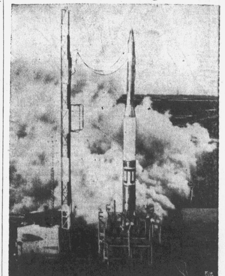
A 72-foot Vanguard, three-stage, test vehicle is shown undergoing simulated flight conditions in photo released by Department of Defense Oct. 5, at Air Force missile center, Cape Canaveral, Fla. With engine being tested in third of series of seven tests, similar rocket will be launched next year carrying U. S. earth satellite. Rocket is also designated as a TV-12. (U. S. Air Force Photo via AP Wirephoto)
