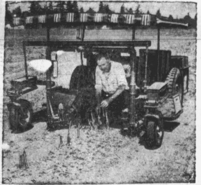
HARVEST HELPER: Stanley Allison demonstrates operation of the machine he designed to put asparagus harvesting on wheels. It enables one man to do the work of eight.
