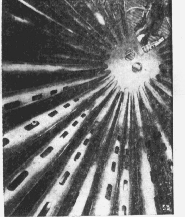
POWER TUBES — Engineer peers down full-scale mockup of pressurized atomic reactor to be installed at Ship-pingport, Pa., for nuclear plant generating electricity. Hafnium metal rods within tubes will control the atom splitting process.
