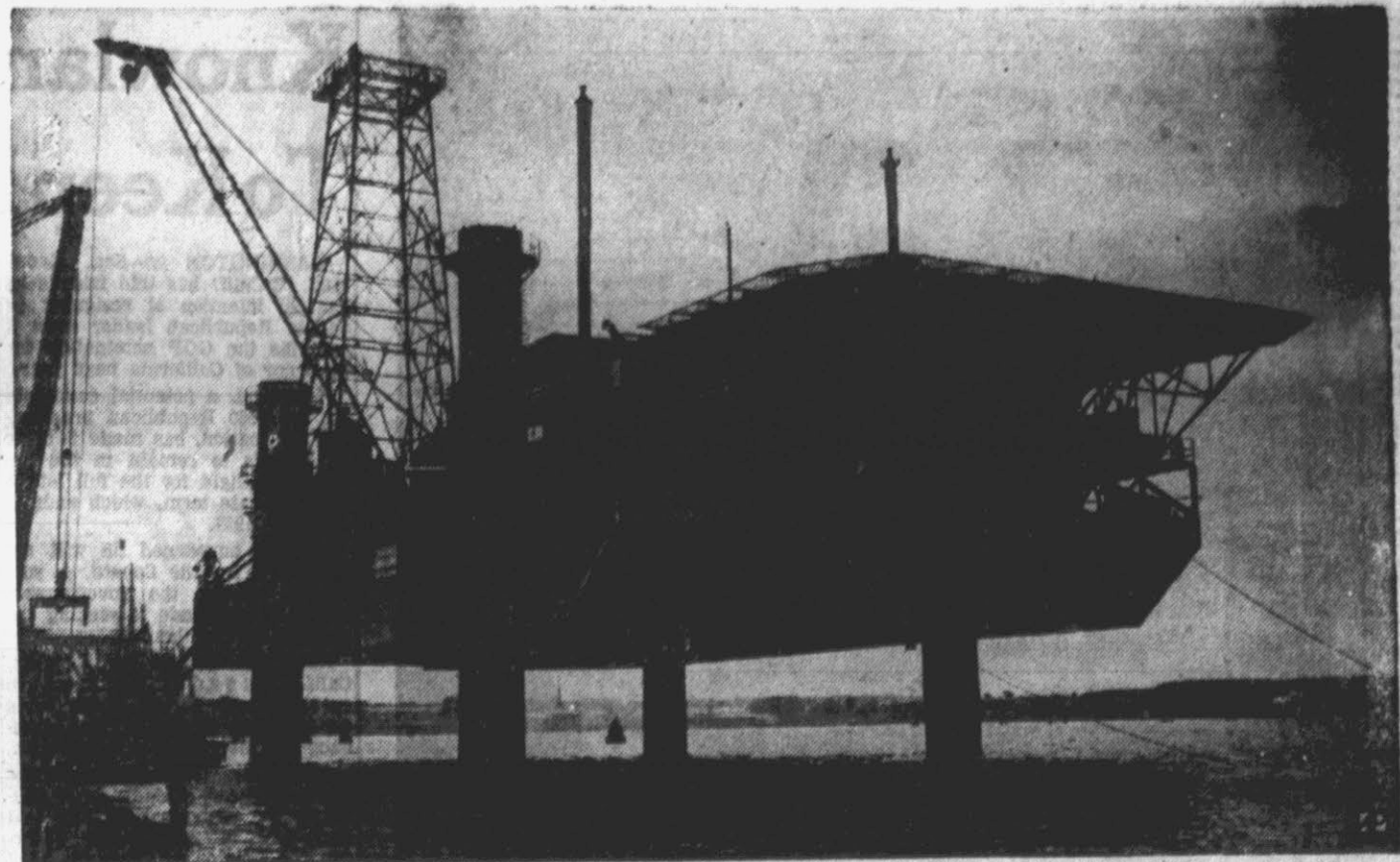
INTERNATIONAL 'ISLAND' — Oil-drilling platform, built at Rendsburg, Germany, for British-French oil interests, is readied for tow to the Persian Gulf. Platform, 220 feet wide and 190 feet long, has drilling tower 180 feet high.
