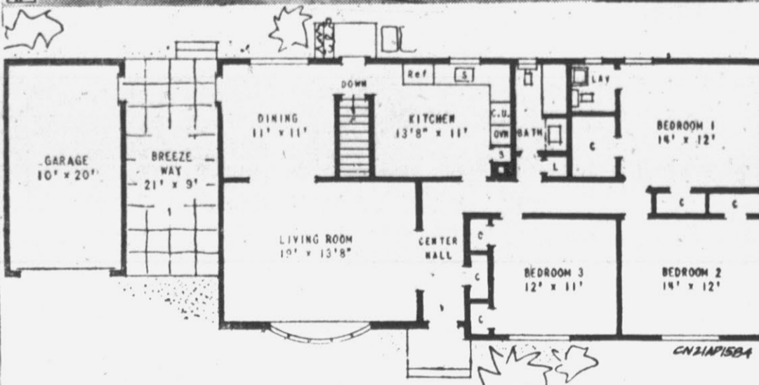
A GRACIOUS living room, separated from the dining area only by a wide inviting arch, is one of the major virtues of this fine three-bedroom home. Over-all dimensions are 74' by 27', including breezeway and garage. It covers 1,458 square feet and is plan CN21AP1584 by Architect Lester Cohen, Room 75, 117 West 48th St., New York 36, N. Y.
