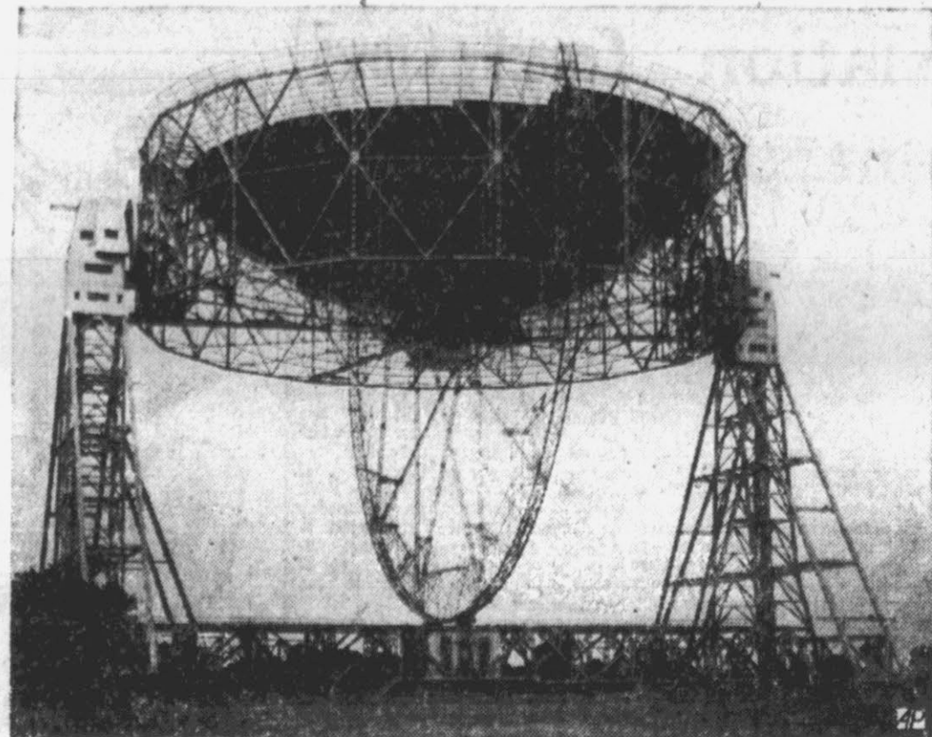
TO SEARCH THE STARS — The new radio telescope at Jodrell Bank, Eng. is ready for use during the International Geophysical Year. The 2,000-ton instrument, straddled on two supports which run on circular tracks, can detect stellar signals from any angle in space.
