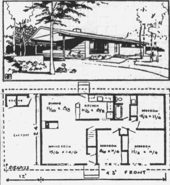
SMALL AND MODERN as tomorrow, this attractive plan offers three bedrooms in only 1,032 square feet of space. A semi-free-standing fireplace divides but doesn't separate living and dining areas. The design is R15AP122 by Architect Jan Reiner, P.O. Box 12, Boston 17, Mass.
