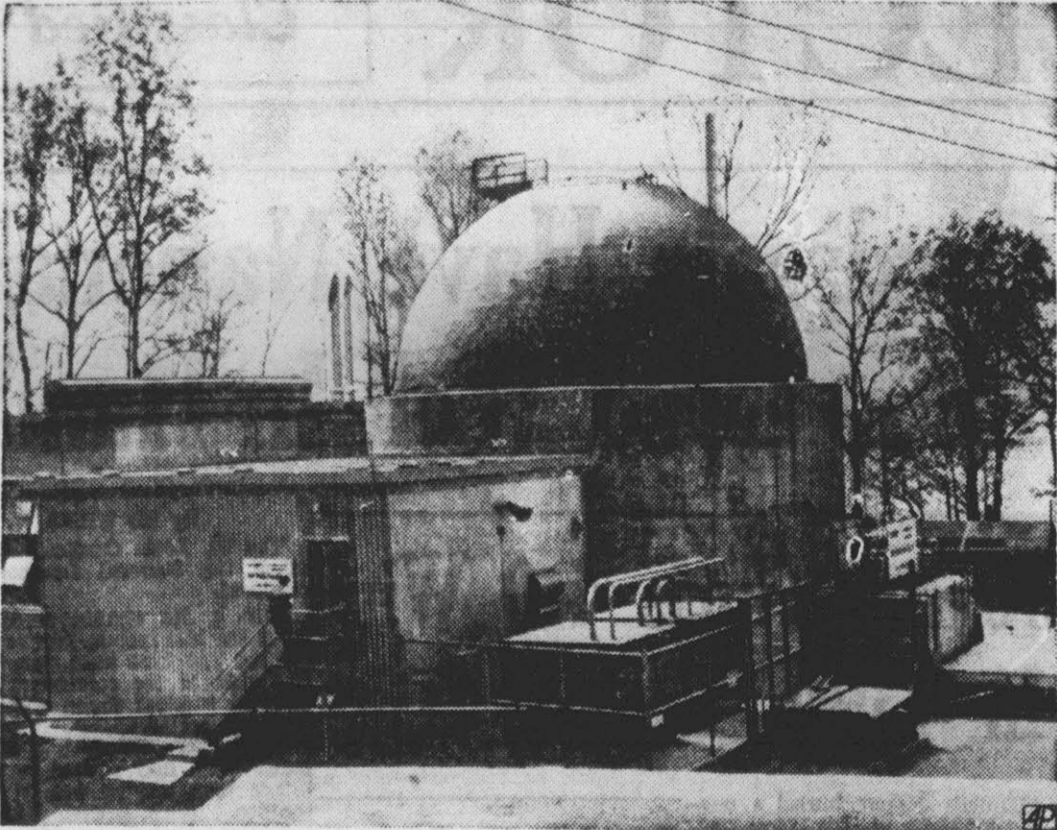
PORTABLE ATOM PLANT — Army's A-power plant with 1855-kilowatt output at Ft. Belvoir, Va., is designed so components can be shipped by air to remote bases such as Arctic.
