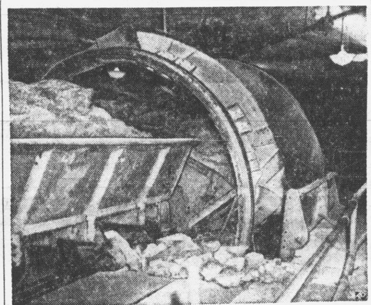
GIANT SALT SHAKER : This huge machine in the International Salt Co.'s at Retsof, N. Y., empties cars automatically by tipping them over.
