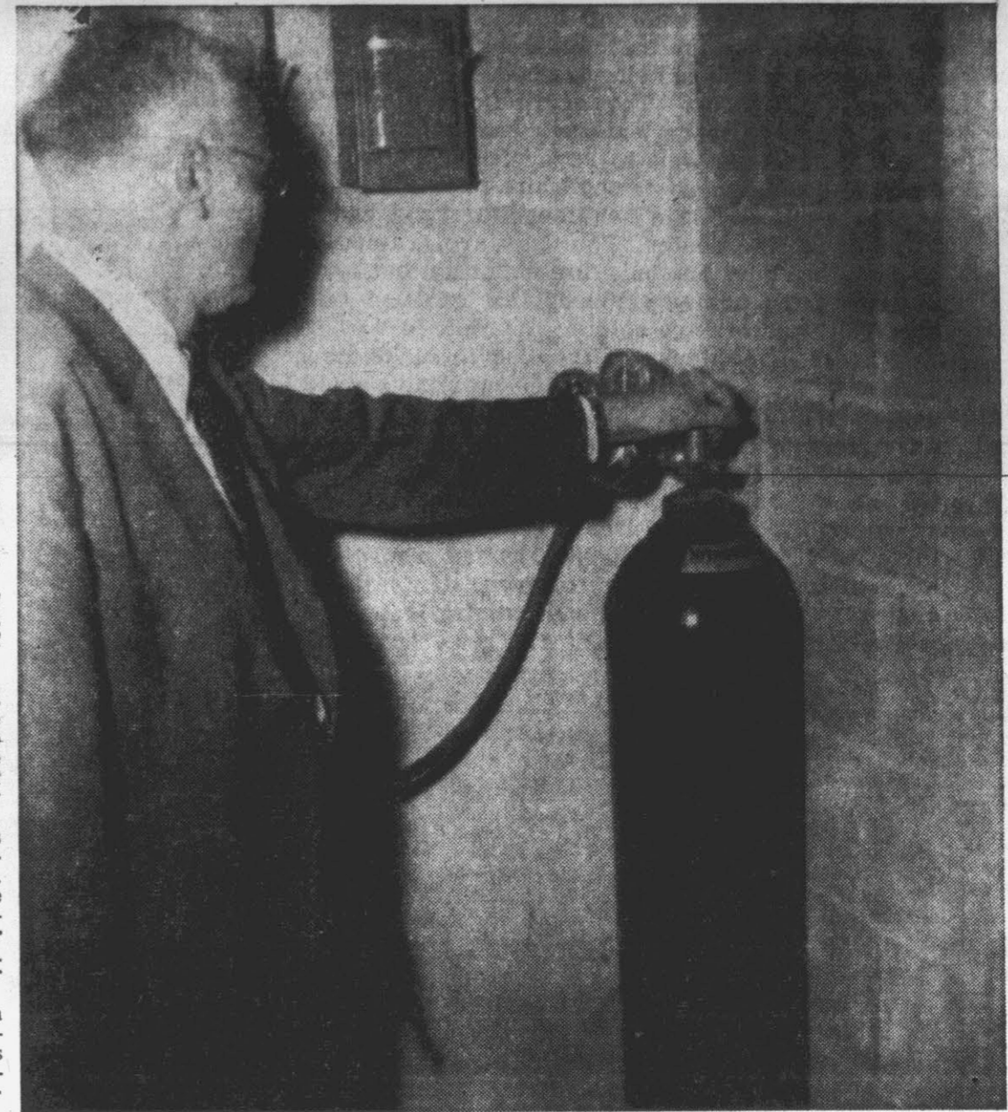
GAS FOR CABLE —Coaxial cable leads from the transmitter to the antenna on the roof of the library. Nitrogen must be fed into the cable to keep it dry. Above Librarian Wendell Smiley adjusts the gas flow which is fed into the line.
