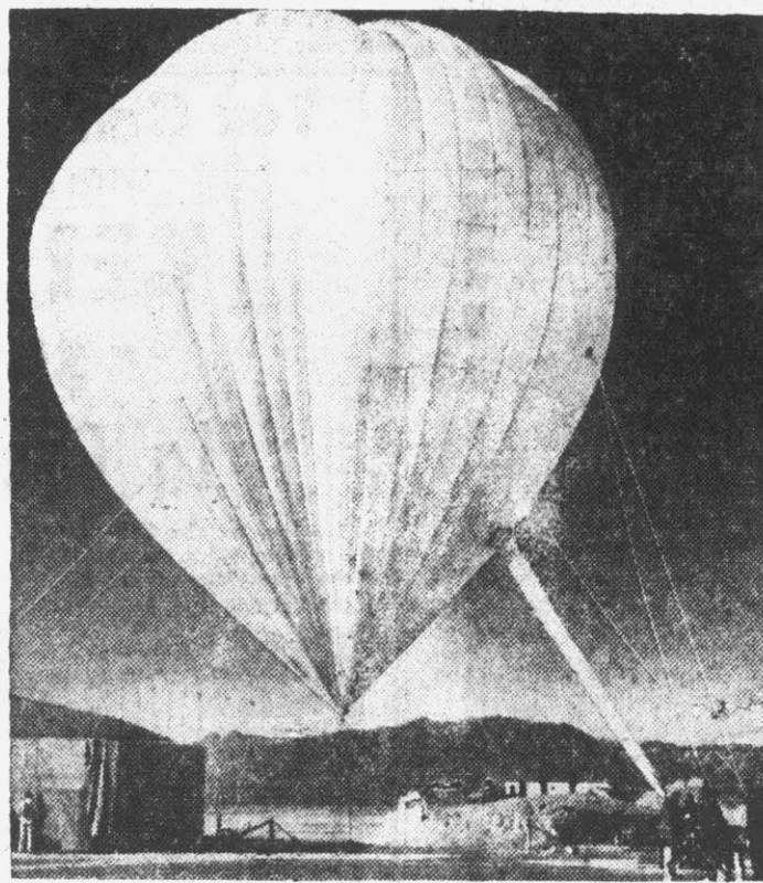
MAY REPLACE TOWER — Helium-inflated balloon is tested by AEC experts near Las Vegas, Nev., to determine its use as an anchored platform to detonate nuclear devices.
