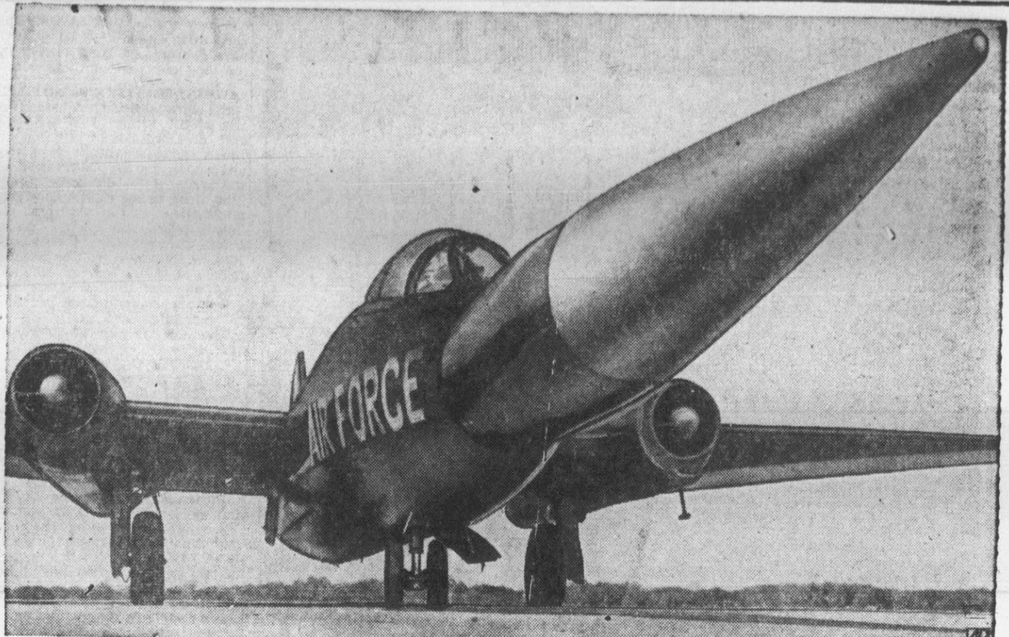
BULLET-NOSED BOMBER —This B57 Canberra jet bomber presents odd, long-nosed appearance after installation of a 17-foot Bomarc guided missile for use in tests. Plane will be used to test the automatic guidance system of the Bomarc.
