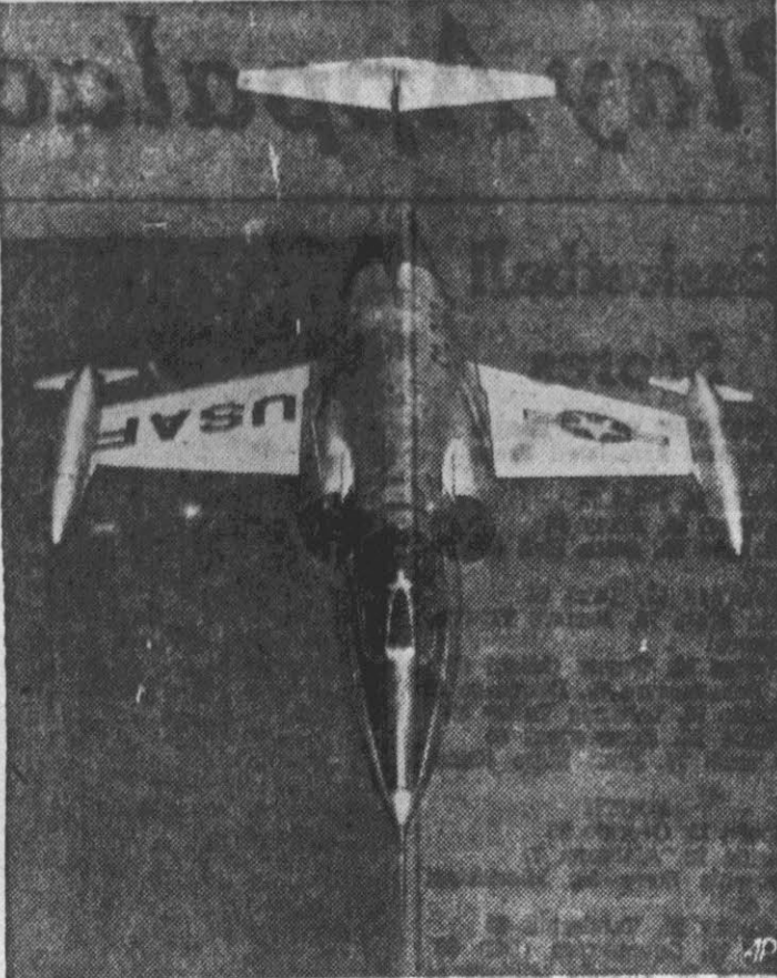
SWIFT SPEEDSTER —This is America's XF-104 Starfighter, believed to be world's fastest fighter jet, which will be used by key continental Air Defense Command units. The 55-foot long plane has wingspread of only 21 feet, 11 inches.
