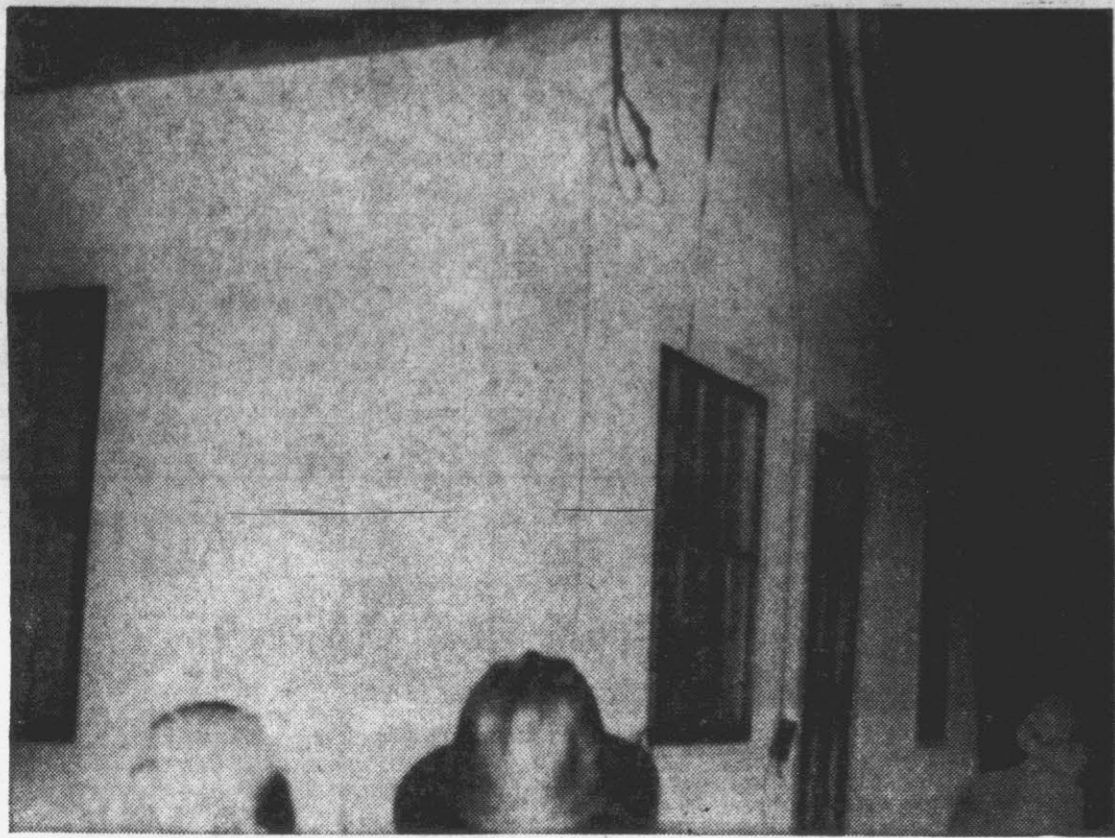
WALL BLOWN OUTWARD—The east wall of a house at 304 Church St. bulged outward as a result of a gas explosion in the basement of the home last night. Inside a large crack in the wall extended the length of the dwelling.
