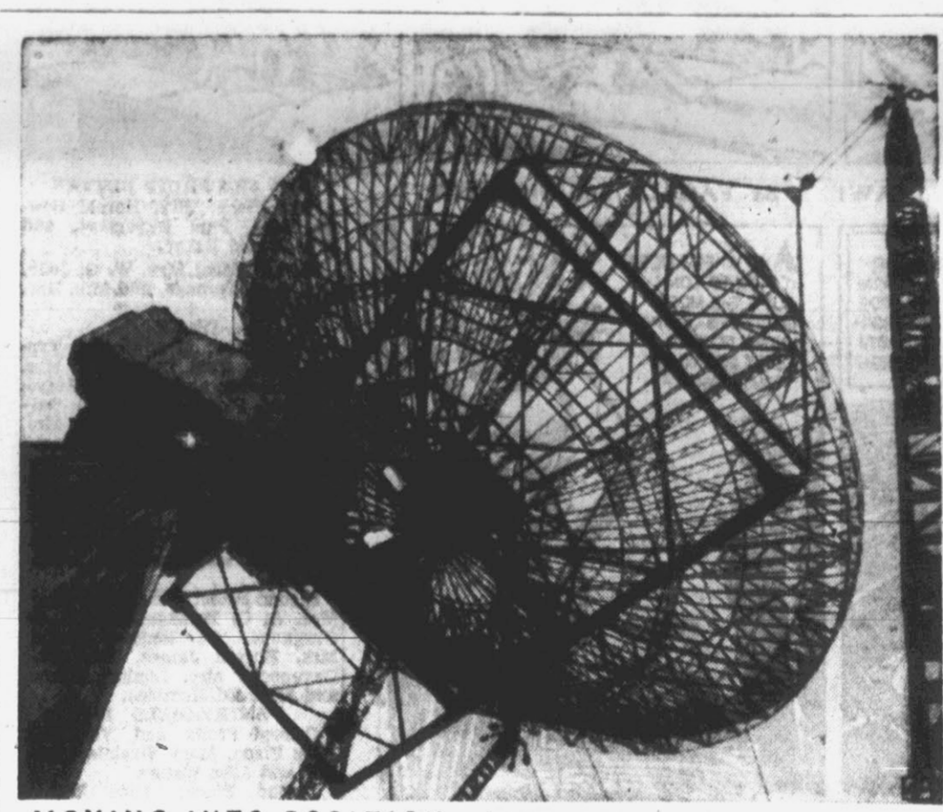
MOVING INTO POSITION — Cranes hoist huge aluminum radiotelescope reflector into place on Stockert Mountain, Germany. It will serve the observatory of Bonn University.
