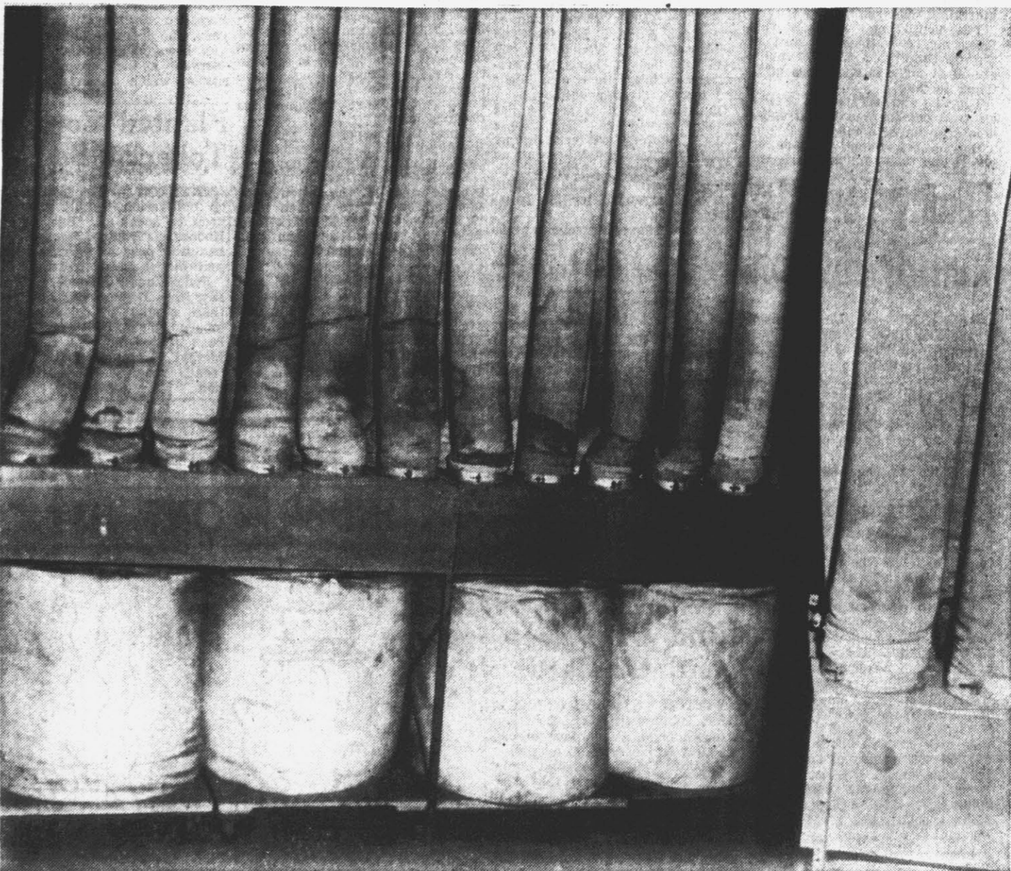
These huge dust bags collect dust and dirt blown from tobacco passing through the stemming operation. The bags, operating like a common vacuum cleaner, have to be emptied every five hours.
