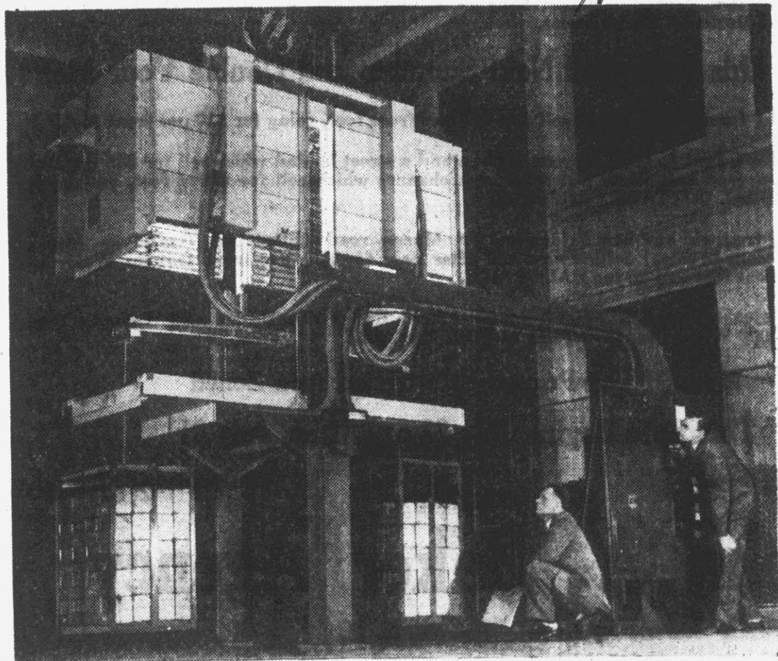
Electric furnace, used to study strength of built-up structures under heating, is lifted to show multi-web beam of aluminum alloy, like beam in plane wing.
