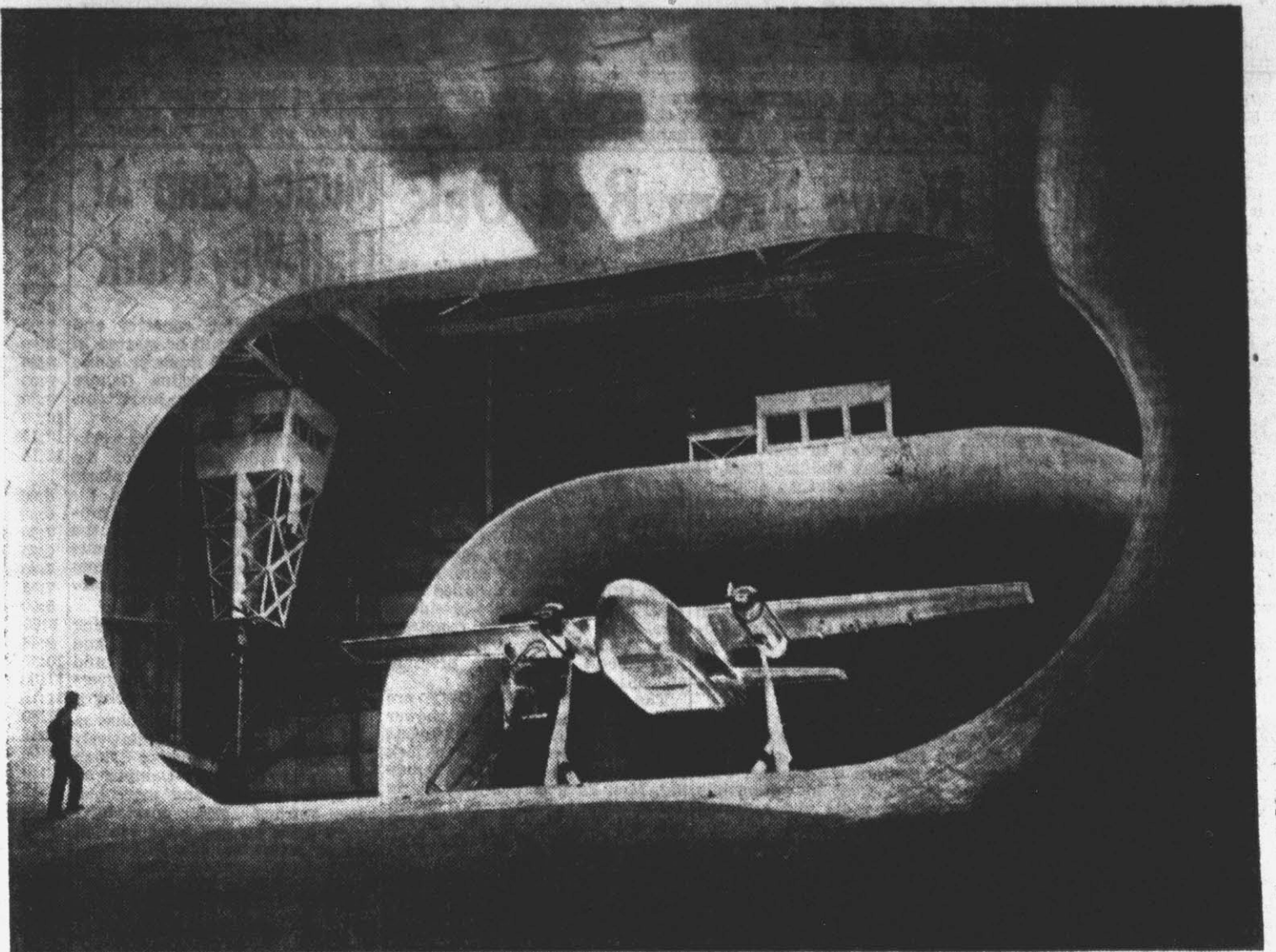
Model of Air Force military cargo plane, the Chase C-123, in full-scale wind tunnel. Scientists are studying plane's aerodynamic characteristics — its stability, control and maximum lift at low speeds.
