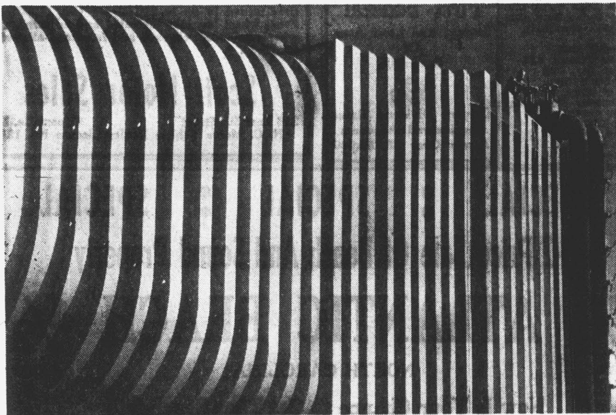
Corner of supersonic pressure wind tunnel, showing heavy steel bracing required to cut down vibration and noise. Vertical black pipes carry water to radiator inside tunnel.
