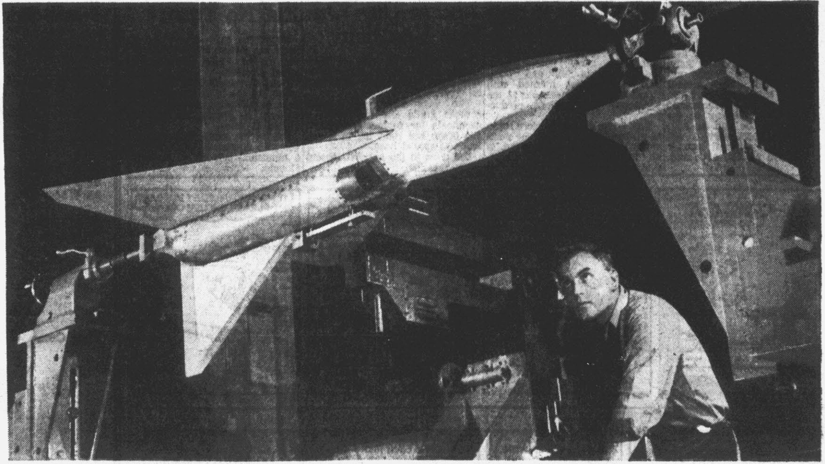
Drag and stability data will be obtained from use of this model of the Convair XF2Y-1 Sea Dart. Later, model will be attached to rocket and fired from NACA's pilotless aircraft research station at Wallop's Island, Va.
