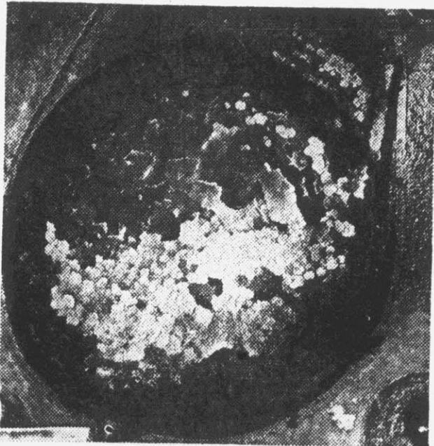
LEAD FOULING —Crusty lead deposits on pistons, after 42,168 miles running with a nationally-sold leaded premium gasoline.
