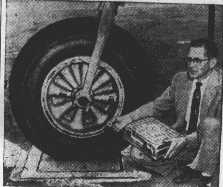
FOR BETTER FLYING—The metal box goes under the plate on which the wheel sits. Inside the box is a little electronic device which gives a continuous record of weight.
