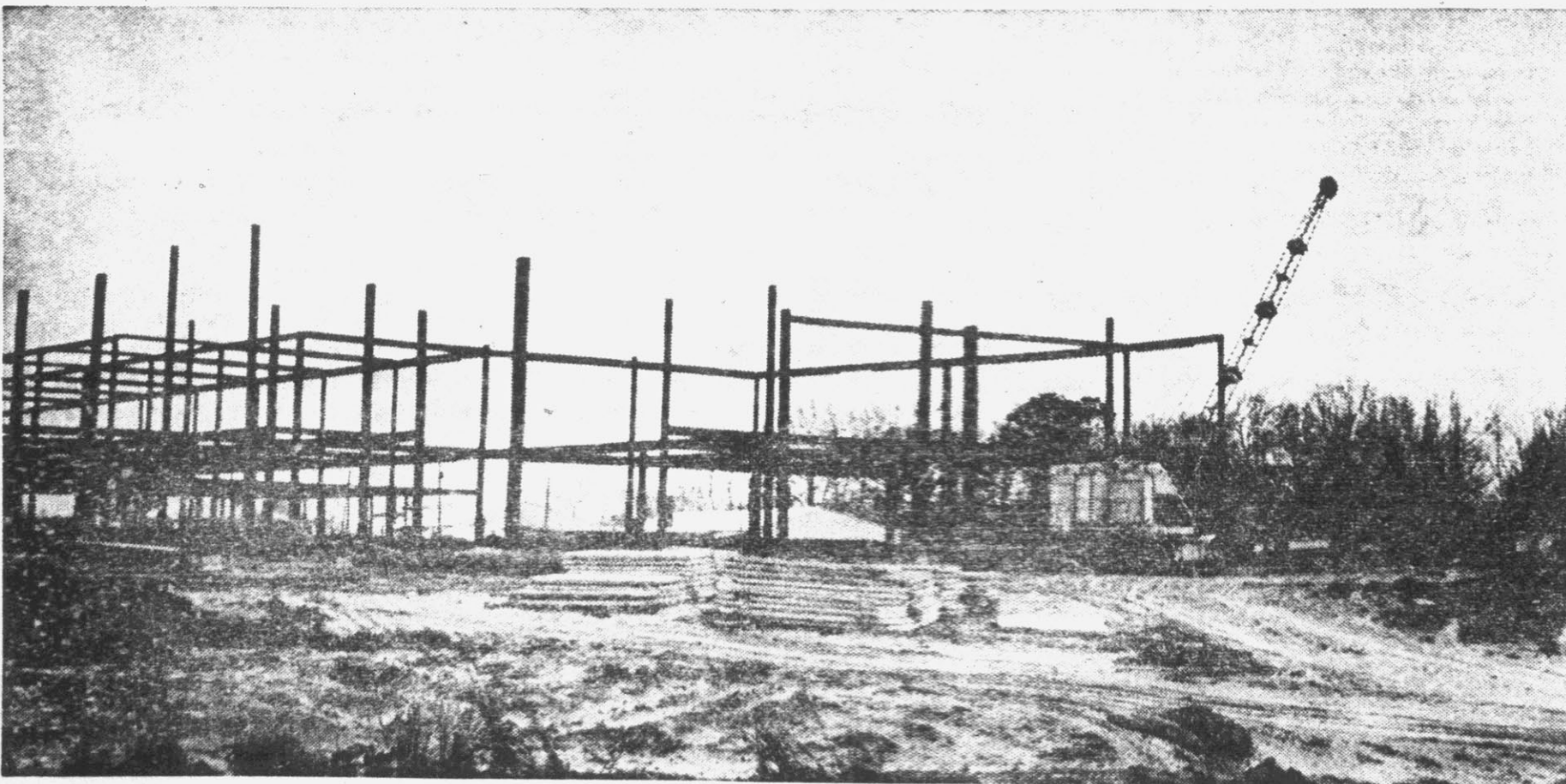
Steel begins to rise at the site of the new high school building on Elm St. The new school is costing $822,855. Facilities will include 15 regular classrooms, three science classrooms, two home economic classrooms, three rooms for the commerce department, two and one-half band rooms, two vocal music rooms, library, kitchen and cafeteria, gymnasium and offices. (Reflector Staff Photo).
