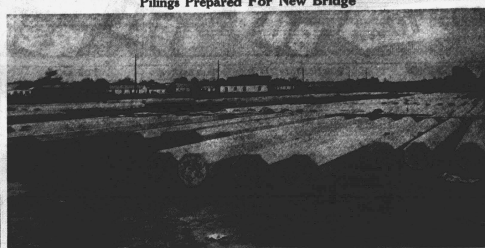
Concrete pilings for the new bridge over the Tar River east of Greenville and ready and waiting for the actual bridge construction to begin. Each of the pilings were poured in special molds and allowed to harden. Later they will be hauled to the bridge site and sunk into the river bed by pile driver. (Reflector Photo by Alvin Taylor).
