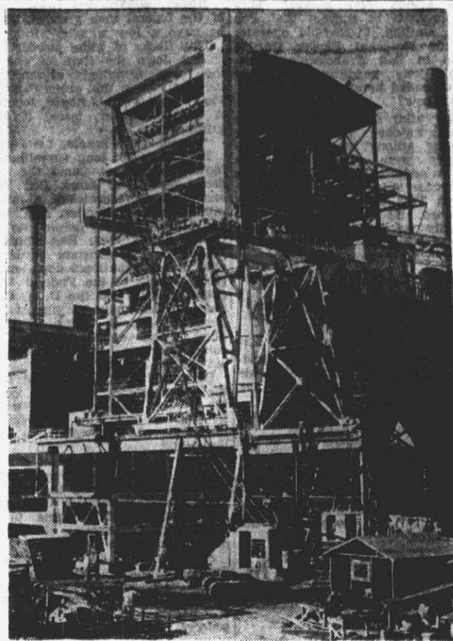
CP&L'S NEWEST AND BIGGEST—A force of 385 workers are rapidly erecting the largest generating unit in Carolina Power & Light Company's system at Moncure. At right is new 200-foot smokestack for "outdoor type" boiler in center. At left is stack for World War II units at Moncure. The new generator is due to begin operation in mid-summer of 1956.
