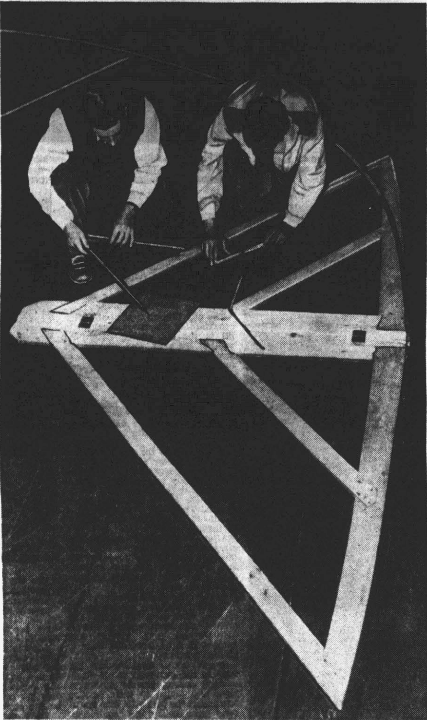
Shapes and sizes of timbers for ship are worked out full scale upon floor. Triangular mockup shows keel and its immediate buttresses.
