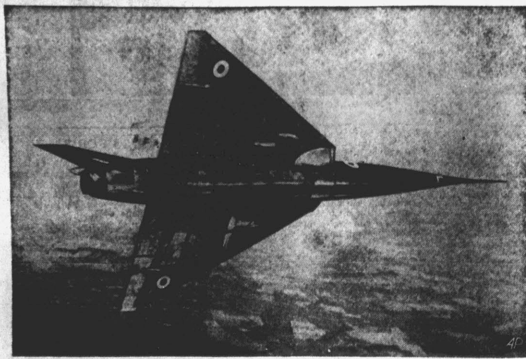
FAIREY DELTA 2 IN FLIGHT—Britain's Fairey Delta 2, shown in flight, will be publicly demonstrated at Farnborough Air Show in England Sept. 5-11. The craft can exceed the speed of sound in level flight over a range of altitudes. It is powered by a Rolls Royce Avon turbojet, and fitted with Fairey powered flying controls. Outstanding feature is the "droop snoot" in which entire nose, including the cockpit, can be lowered by the pilot to improve the forward view for takeoff and landing. (AP Wirephoto)
