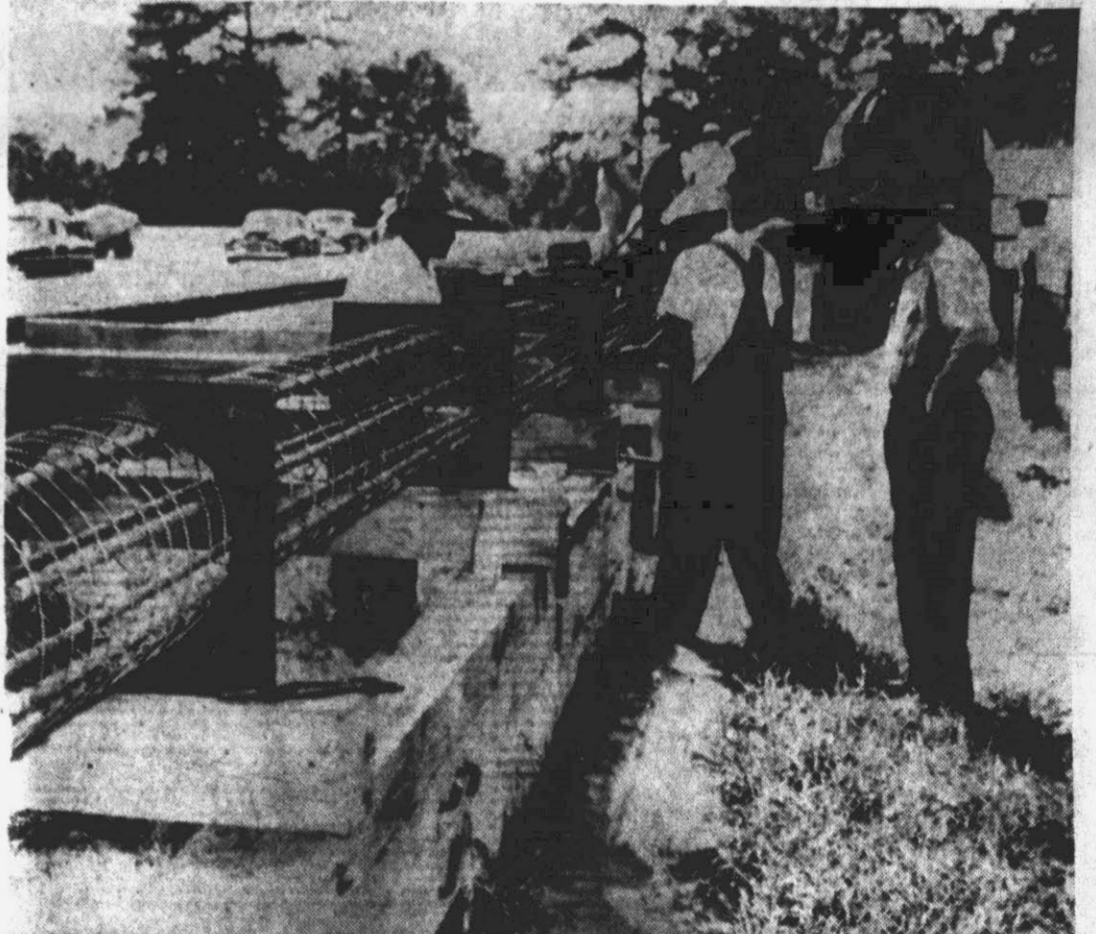
These steel rods form the skeleton for the pilings which are to be sunk under the new bridge. After workmen have completed the job of wiring the rods together they will be placed in steel forms and concrete poured around them.
