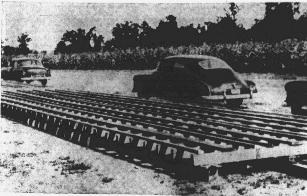
Metal forms in which the concrete pilings are poured are set up on wooden bases, one of which is shown above. These bases were constructed some time ago by bridge crews. The crews have set up the site alongside the fill now being constructed to the river bank.
