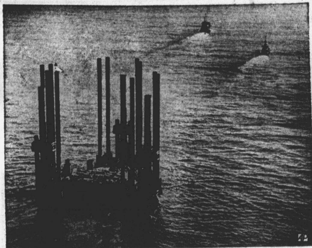
ON SCHEDULE —The 6,000-ton Texas-tower type "Island" which will be offshore radar station in continental defense system is towed toward permanent location on George's Bank, 100-odd miles off the New England coast. Ocean-going tugs are Marion Moran, left, and M. Moran.
