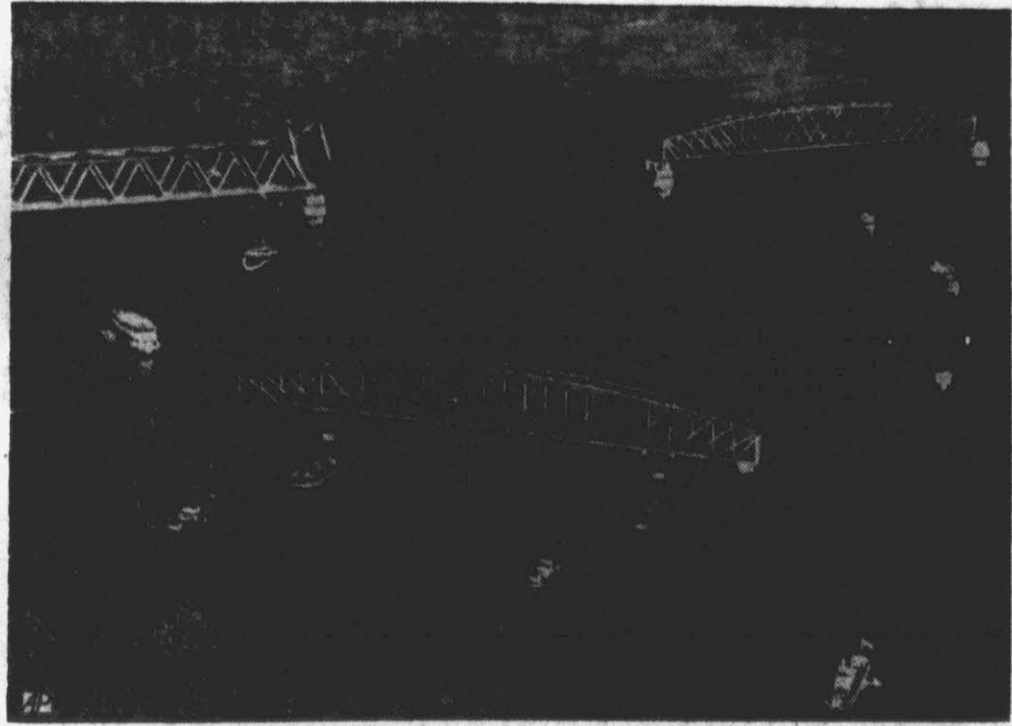
BRIDGING THE GAP—Rebuilding of the Moerdyk railway bridge over Holland's Diep River nears completion as a span is towed into place in the gateway to Belgium and France.
